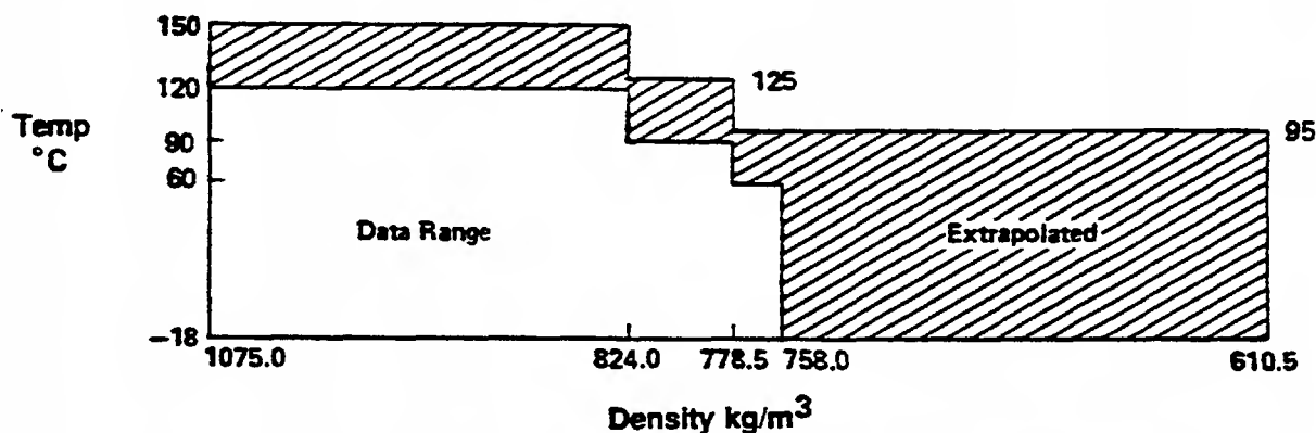
Figure VII-1 — Data Limits for TABLE 53A, Generalized Crude Oils
