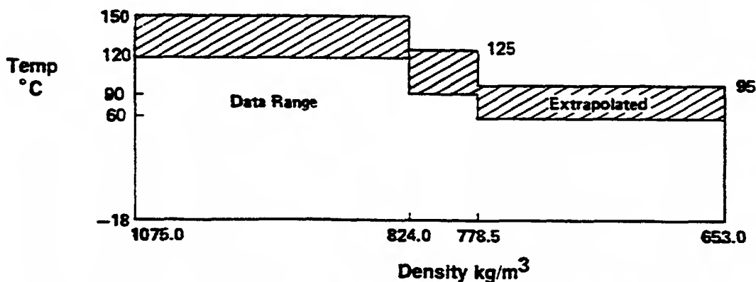
Figure VII-2 — Data Limits for TABLE 53B, Generalized Products
