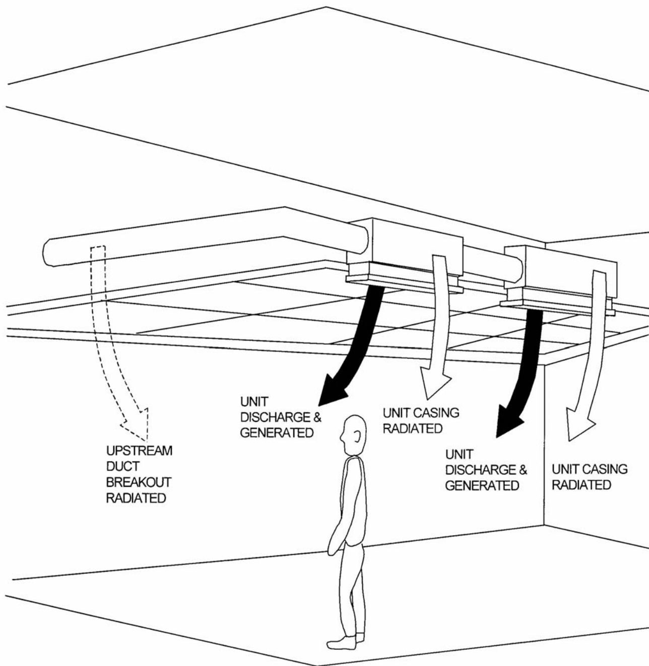
Figure 3. Integral Diffuser Terminal Acoustic Model
