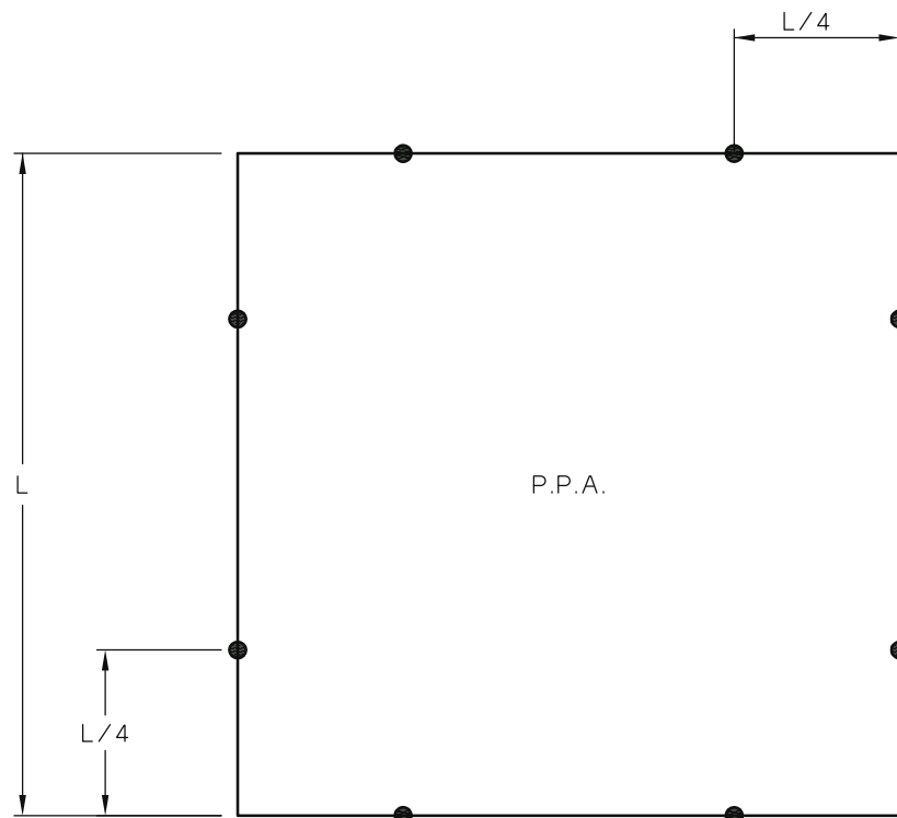
FIGURE 4 OBSERVER POSITIONS FOR GLARE CALCULATIONS
