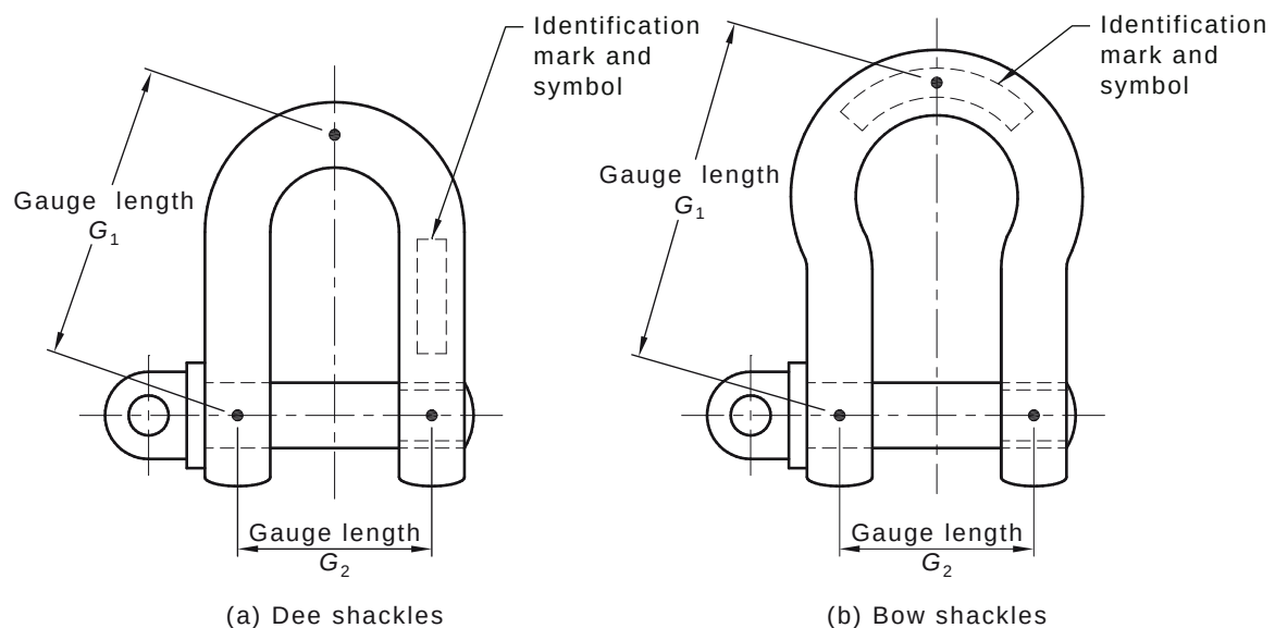
FIGURE 1 TYPICAL POSITIONS FOR MARKING SHACKLES
