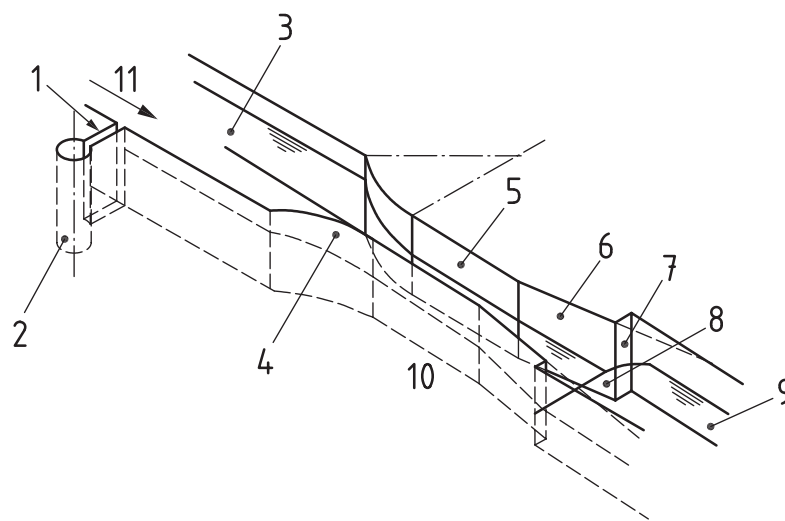
a) Isometric of level-invert rectangular-throated flume ( p = 0 )
