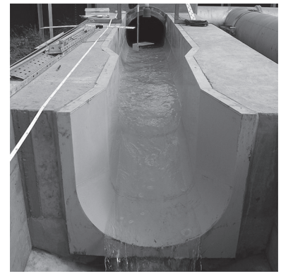
c) U-throated flume
