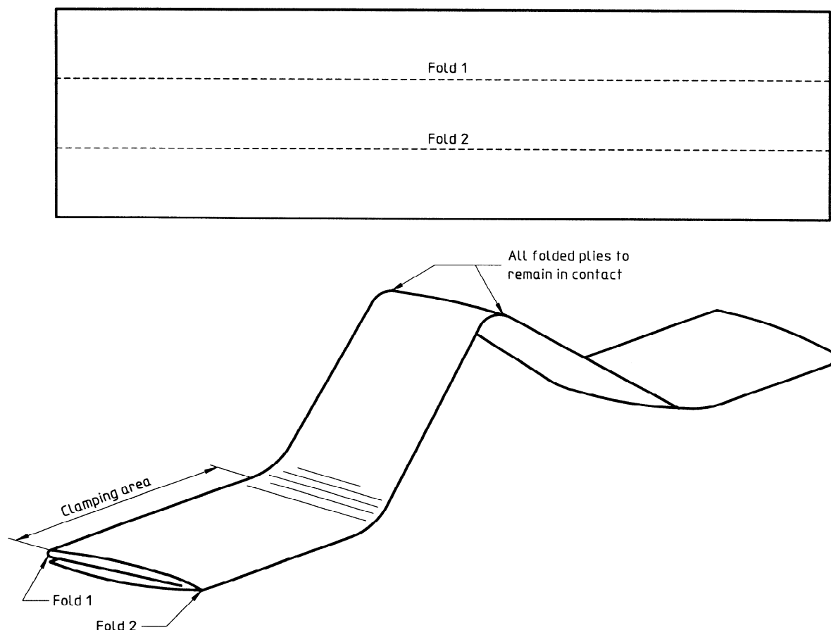
Figure 1 — Illustration of folding and configuration of test piece for De Mattia method
