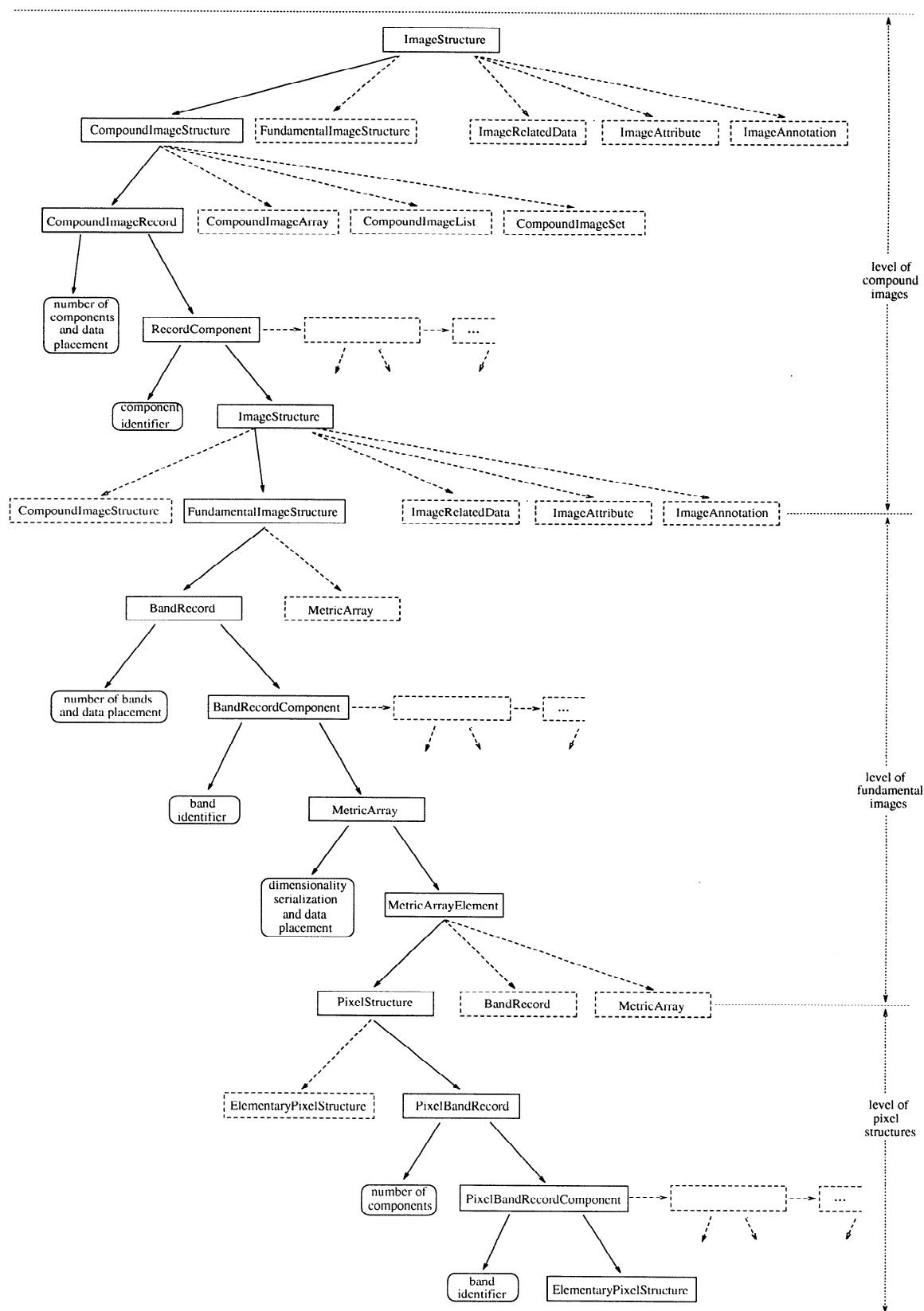
Figure 4 - Representation of image structures within the IIF-DF syntax.
