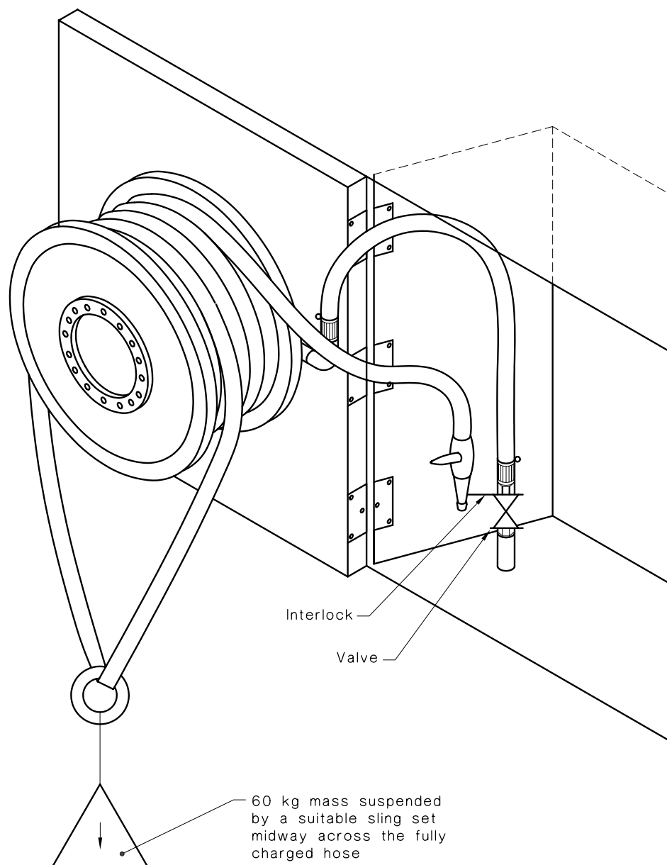
FIGURE C1 DETAILS OF LOAD TEST FOR SWING ARM TYPE HOSE REELS
