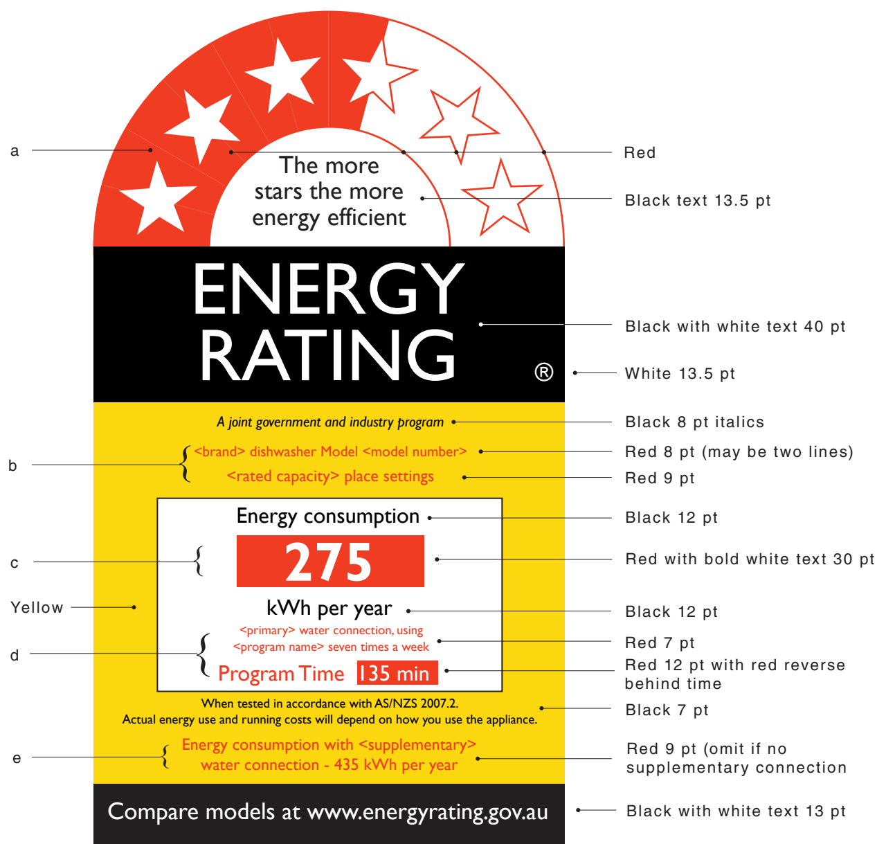
Figure 5.1 — Example of base energy rating label elements
