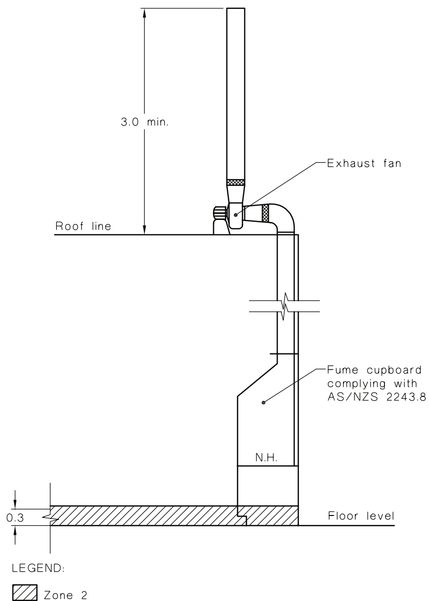
FIGURE 5.1 FUME CUPBOARD COMPLYING WITH AS/NZS 2243.8 AND LABORATORY FLOOR LEVEL
