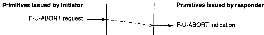
Figure 5 — F-U-ABORT service
