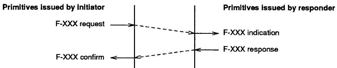
Figure 4 — Confirmed service
