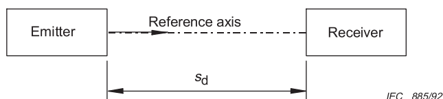
Figure 1a - Type T, emitter and receiver - Trough beam photoelectric
