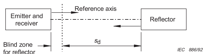
Figure 1b - Type R, emitter-receiver and reflector - Retroreflective photoelectric
