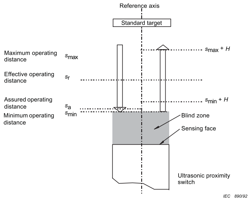
Figure 4 – Relationship between operating distances of ultrasonic proximity switches (see 4.2.2, 7.2.1.3 and 8.4.1)
