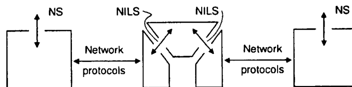
B. Network layer elements only, with relaying component separated
