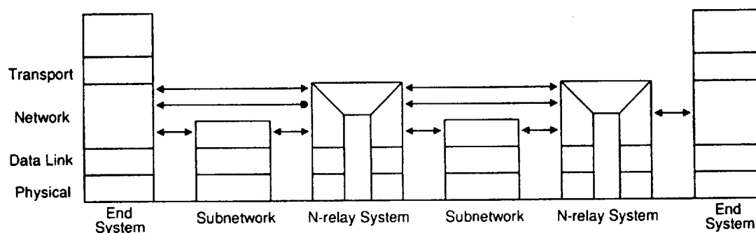
A. Full architectural model (ISO 8648)
