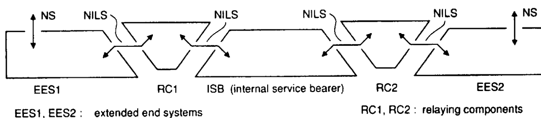
B. Network layer service-level representation
