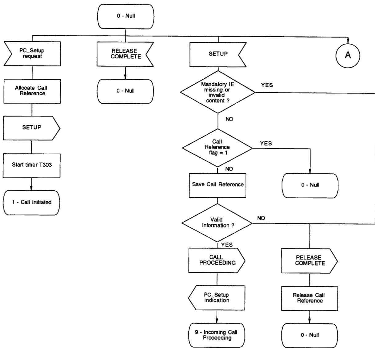
Figure 9 — Connection oriented Protocol Control SDL (Sheet 1 of 10)
