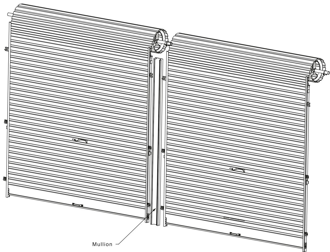
FIGURE 4.2 TYPICAL MULLION
