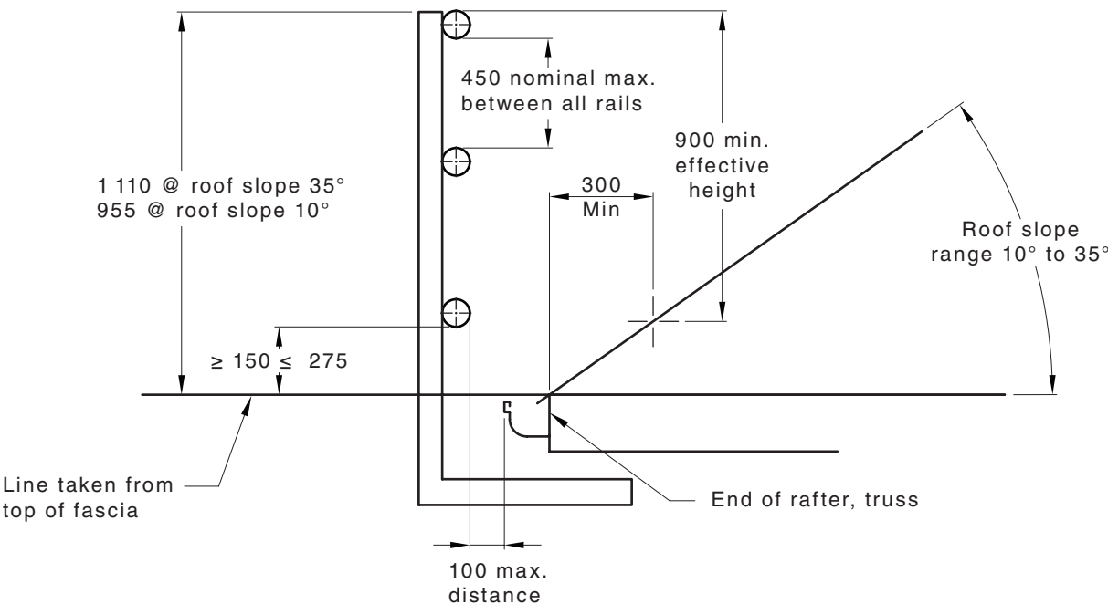
Figure 4.1 — Effective height of a guardrail — Guardrail is outside the roof edge
