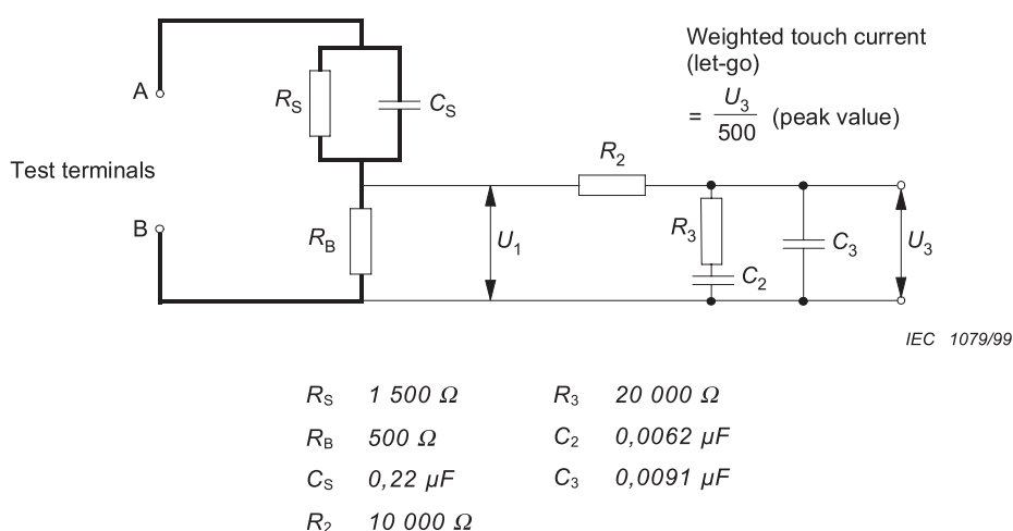
Figure 5 – Measuring network, touch current weighted for let-go
