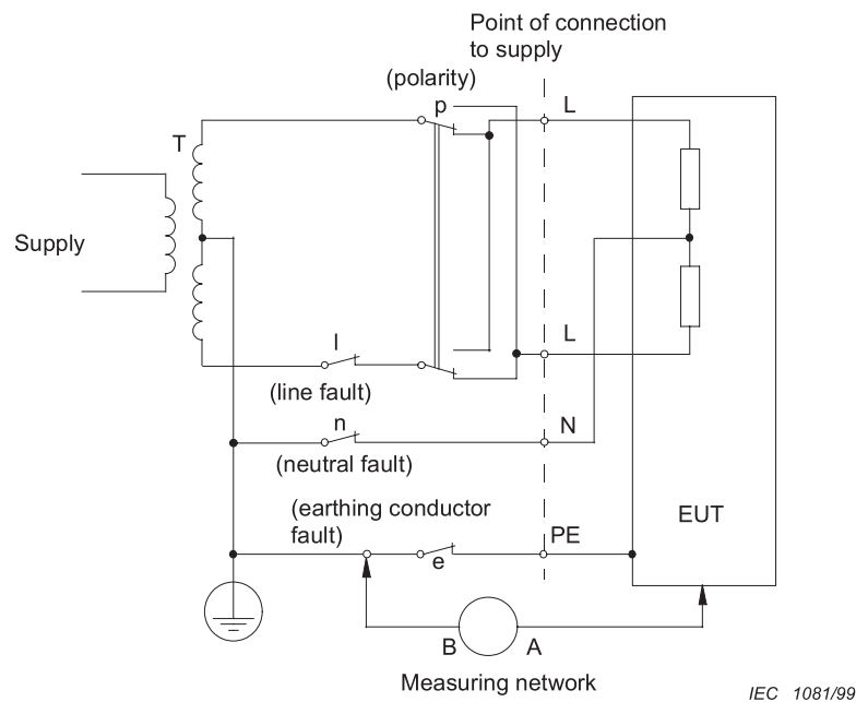
Figure 7 – Test configuration: single-phase equipment on centre-earthed TN or TT system
