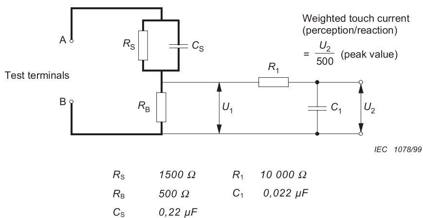
Figure 4 – Measuring network, touch current weighted for perception or reaction
