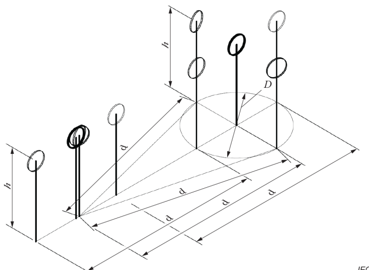
b) H_y validation measurement with loop antennas
