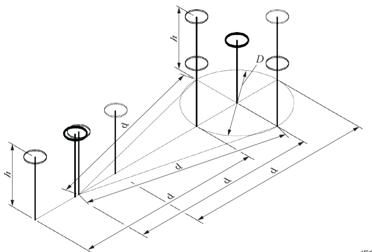
c) H_z validation measurement with loop antennas
