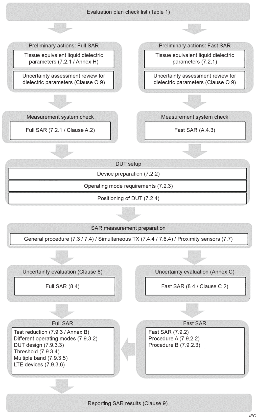
Figure 1 – Quick start guide
