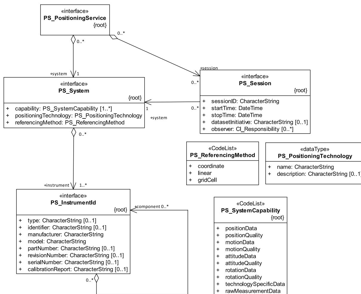
Figure 4 — UML diagram — PS_System and PS_InstrumentId classes
