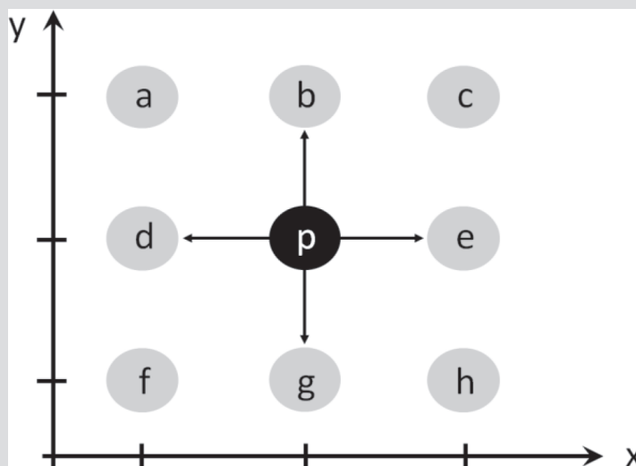
Figure 3 — Sample grid neighbourhood
