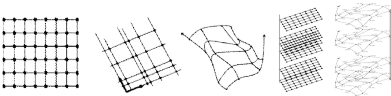
Figure 2 — Sample regular and irregular grid structures (ISO 19123-1)
