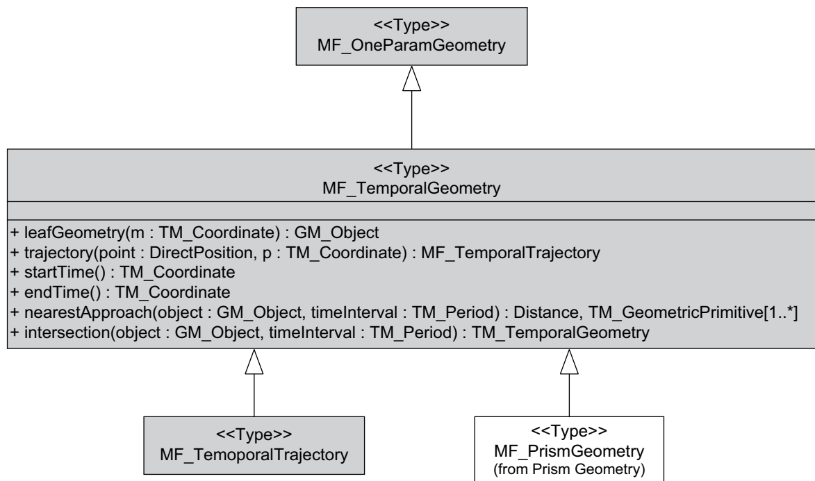
Figure 6 — Context Diagram: MF_TemporalGeometry
