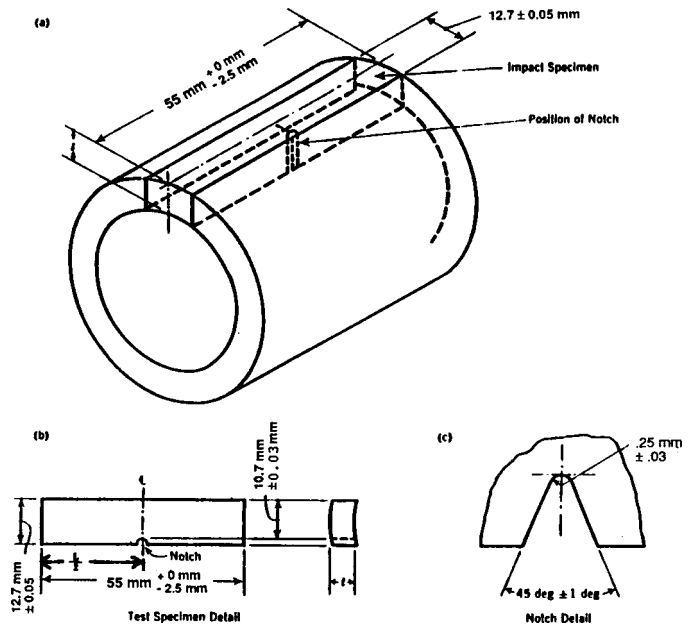
FIG. 2 Impact Test Specimen for Ductile Iron Pipe and Tube
