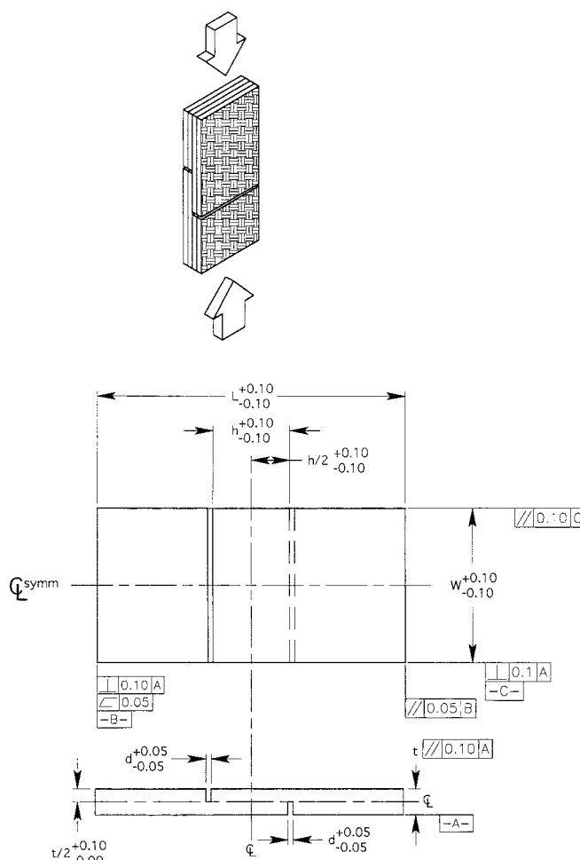
FIG. 2 Schematic of Double-Notched Compression Specimen
