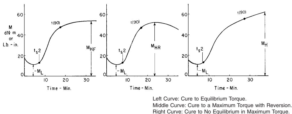
FIG. 1 Types of Cure Curve
