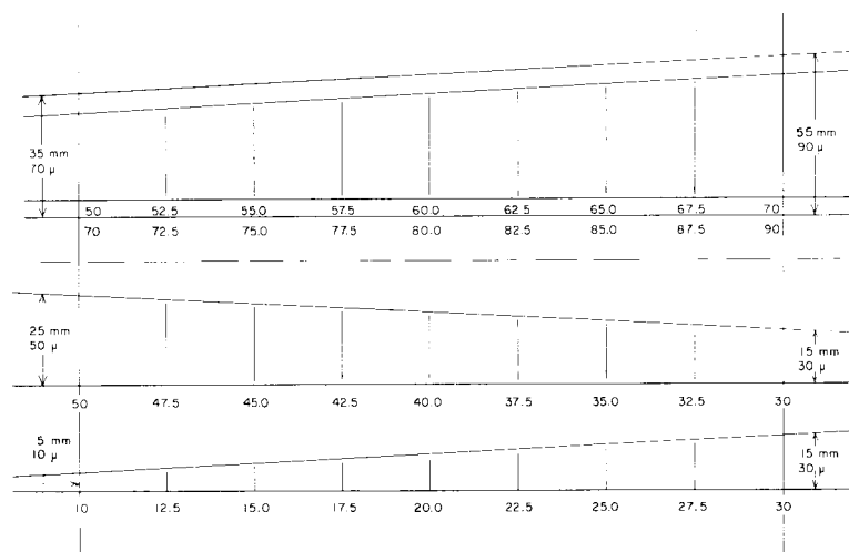
FIG. 3 Wedge Scale
