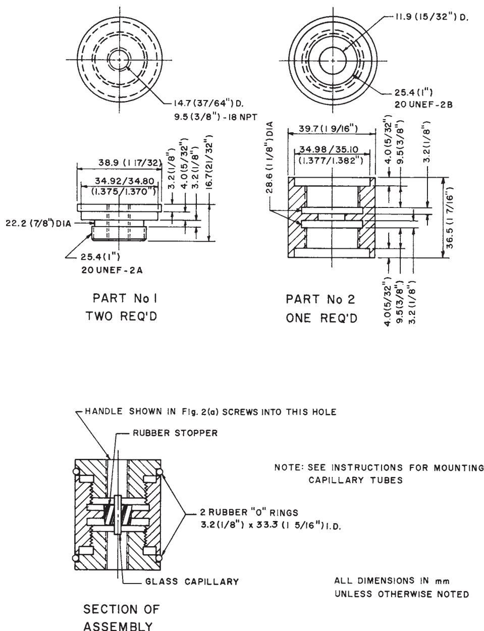
FIG. 1 Capillary Tube Holder
