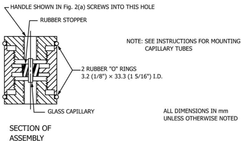
FIG. 1 Capillary Tube Holder
