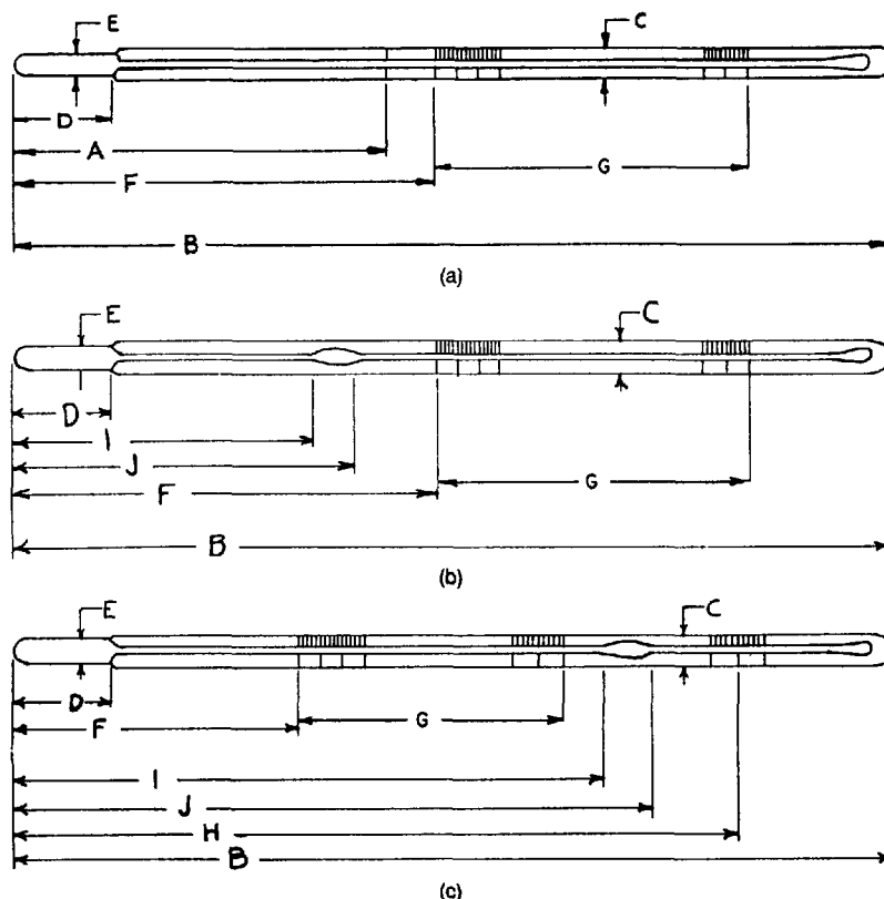
FIG. 1 Thermometer Designs
