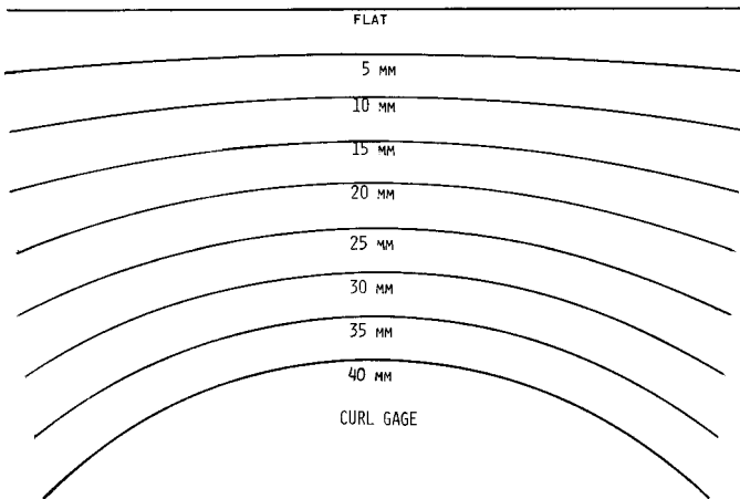
NOTE 1—Not to scale. FIG. 1 Curl Gauge
