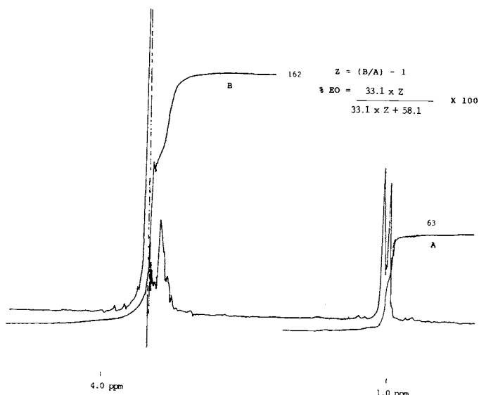
FIG. 1 ^1\text{H} NMR Spectrum of a Polyol Containing 45% EO
