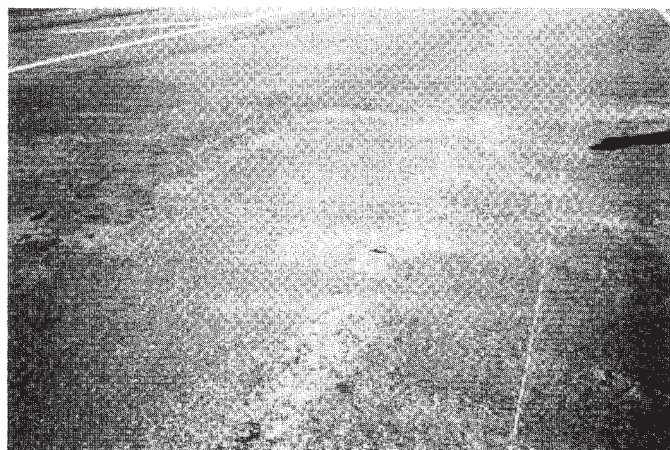
FIG. X1.22 Medium-Severity Corrugation
