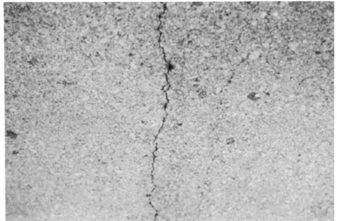
FIG. X1.37 Low-Severity Longitudinal Crack
