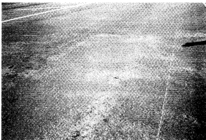
FIG. X1.22 Medium-Severity Corrugation
