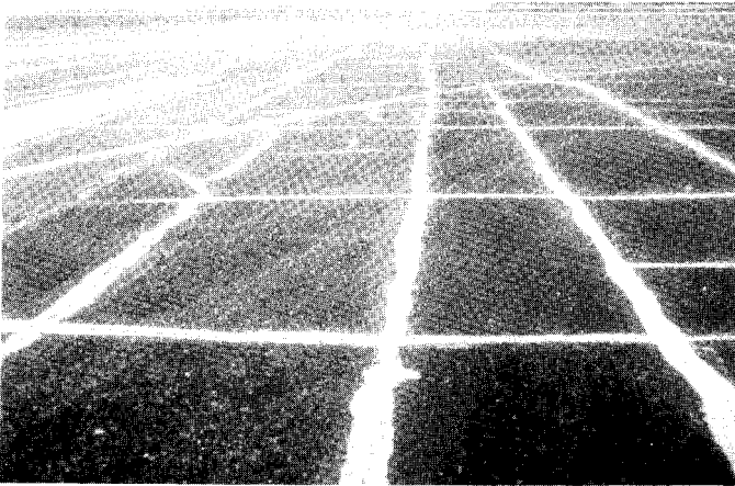
FIG. X1.13 Low-Severity Block Cracking, Filled Cracks
