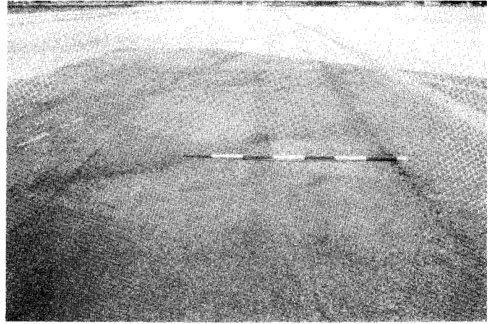
FIG. X1.25 Medium-Severity Depression (1 1/2 in. (37.5 mm))
