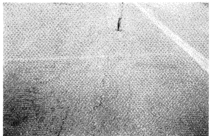
FIG. X1.1 Low-Severity Alligator Cracking
