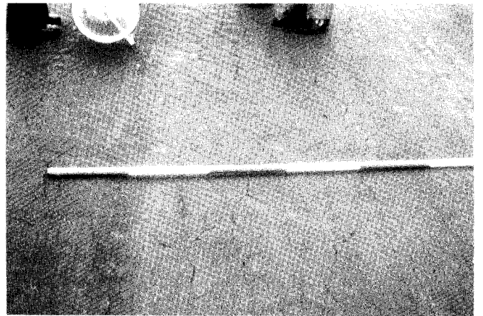
FIG. X1.6 Medium-Severity Alligator Cracking
