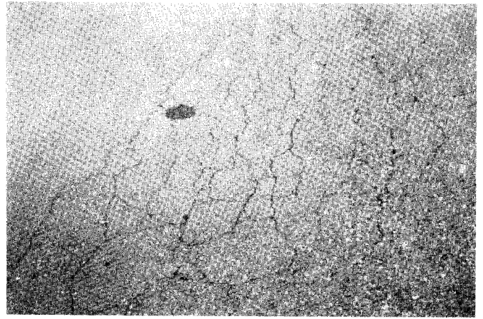
FIG. X1.5 Medium-Severity Alligator Cracking
