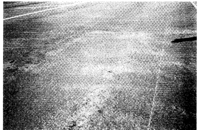
FIG. X1.22 Medium-Severity Corrugation
