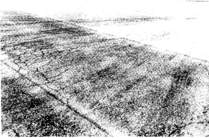
FIG. X1.8 Medium-Severity Alligator Cracking, Approaching High Severity (Example 2)
