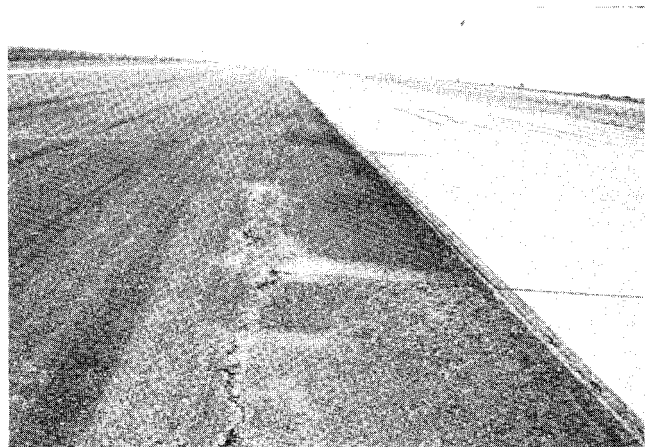
FIG. X1.41 Medium-Severity Longitudinal Crack
