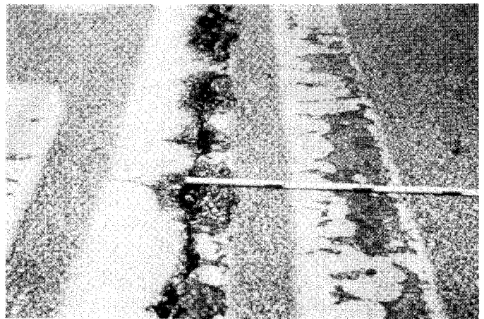
FIG. X1.36 High-Severity Joint Reflection Cracking
