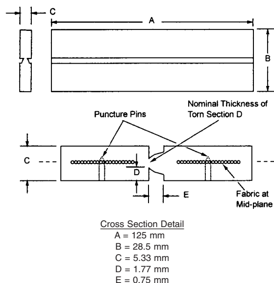
FIG. 3 Schematic diagram of "Constrained Path" tear test piece (1)
