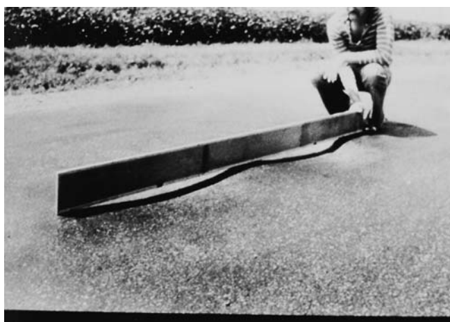
FIG. X1.15 High-Severity Corrugation
