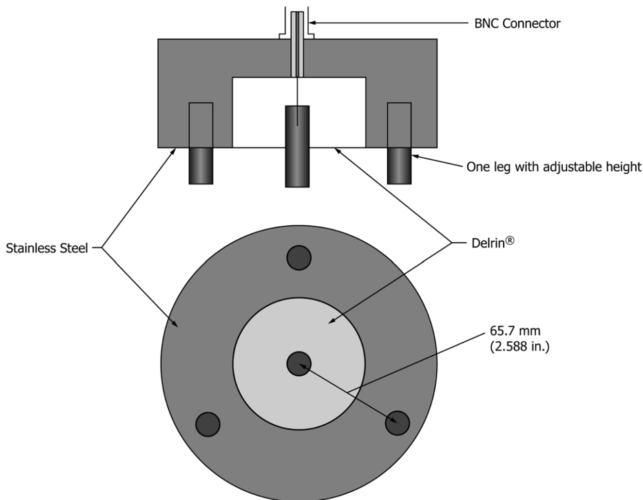
FIG. 3 Coaxial Head (CH)
