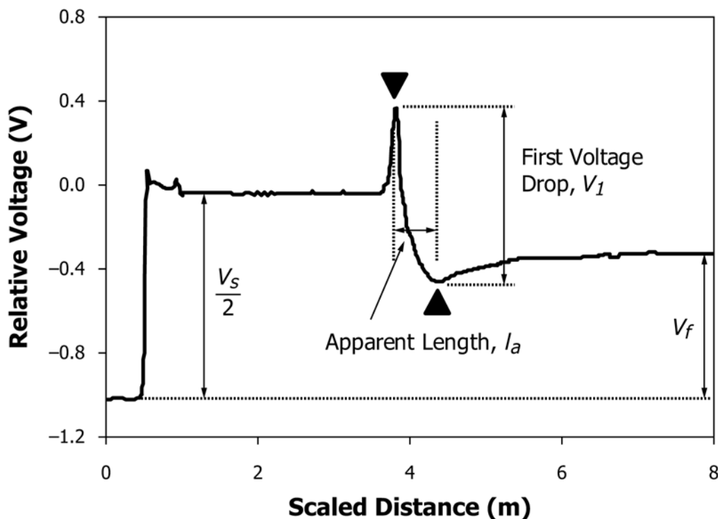
FIG. 1 Typical TDR Waveform for Soil Showing Measurements to Obtain Apparent Dielectric Constant, K_a , Bulk D.C. Electrical Conductivity, EC_b , First Voltage Drop, V_1 , and Long Term Voltage, V_f .
