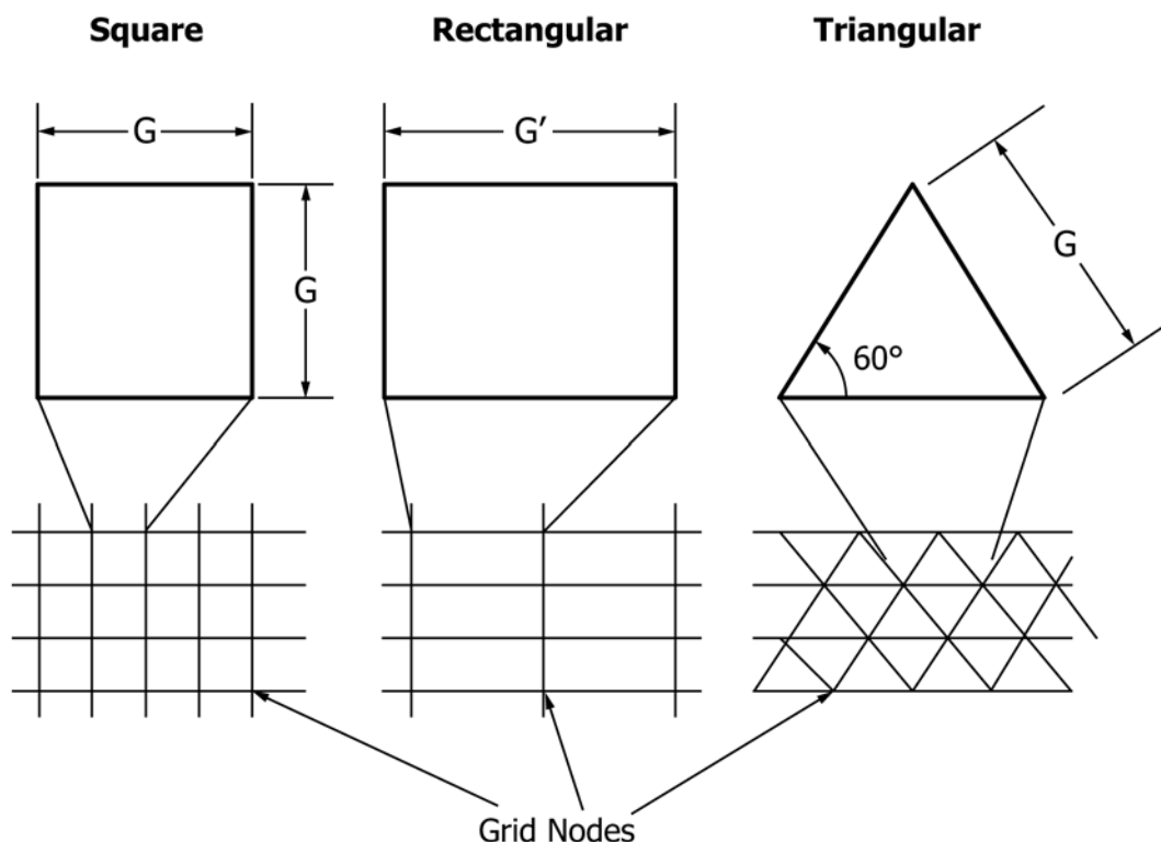
FIG. 2 Grid Patterns for Detecting Hot Spots. Borings are Made at the Grid Nodes
