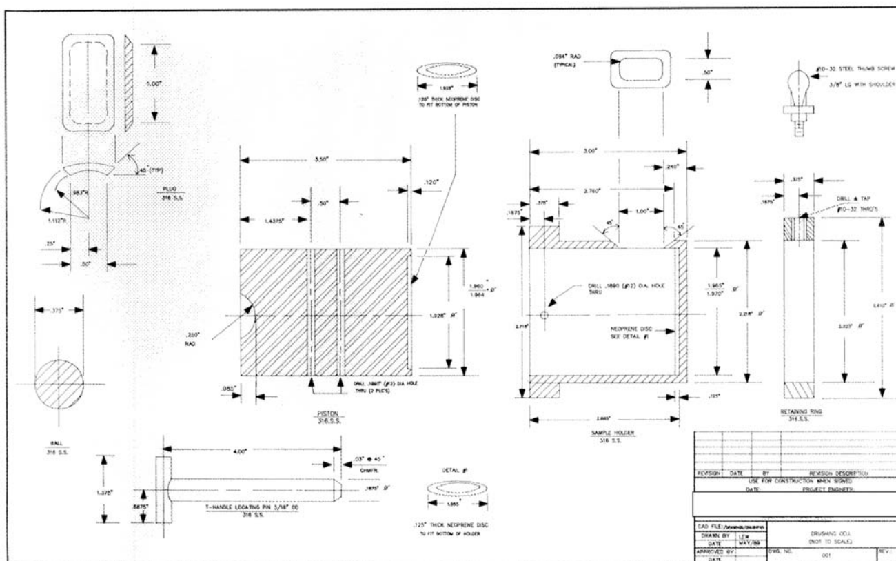
FIG. 1 Test Cell
