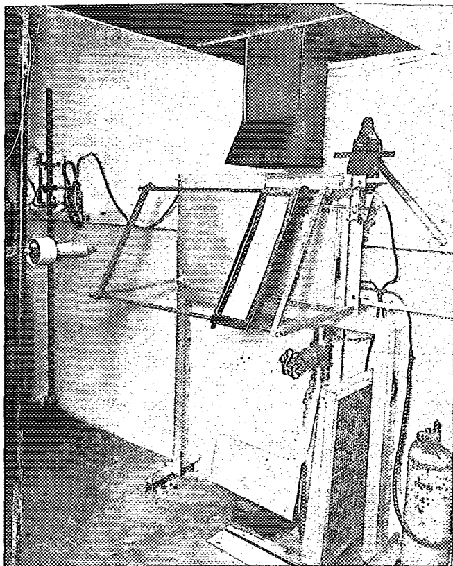
FIG. 1 Radiant Panel Flame Spread Test Equipment
