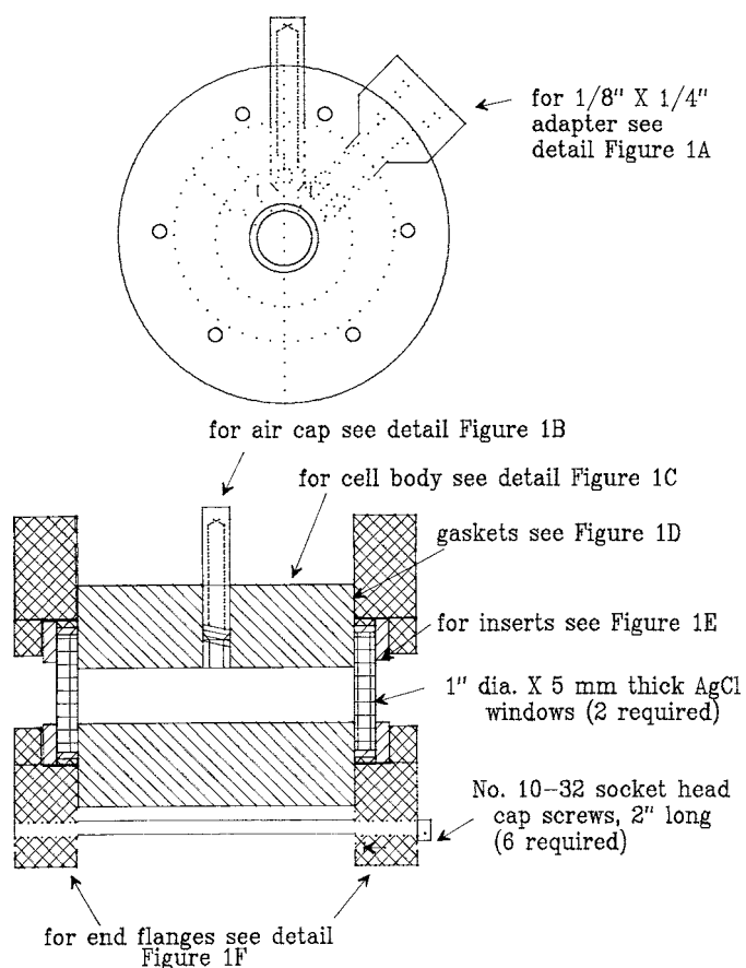
FIG. 1 Infrared Cell
