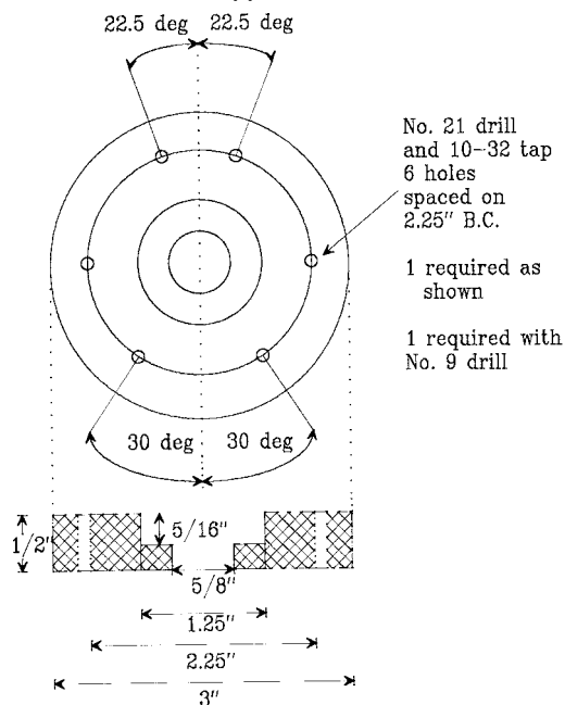
FIG. 1(f) Flange Detail
