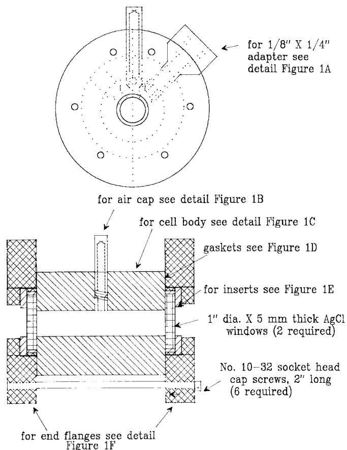
FIG. 1 Infrared Cell
