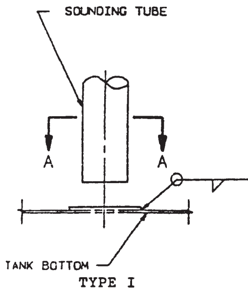
FIG. 1 Type I Sounding Tube
