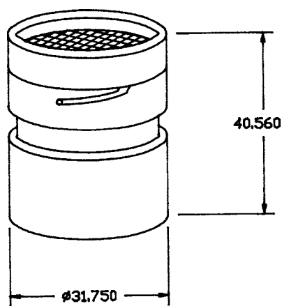
FIG. 1 Sample Cell
