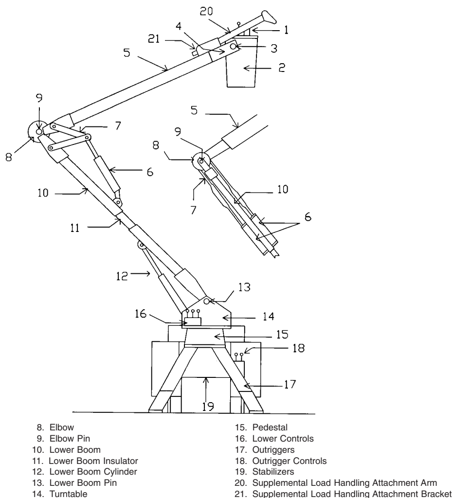
FIG. 1 Articulating-Boom APD Nomenclature Diagram
