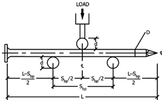
FIG. 2 Load and reaction bearing point positions for smooth-shank and fully deformed-shank nails and spikes.
