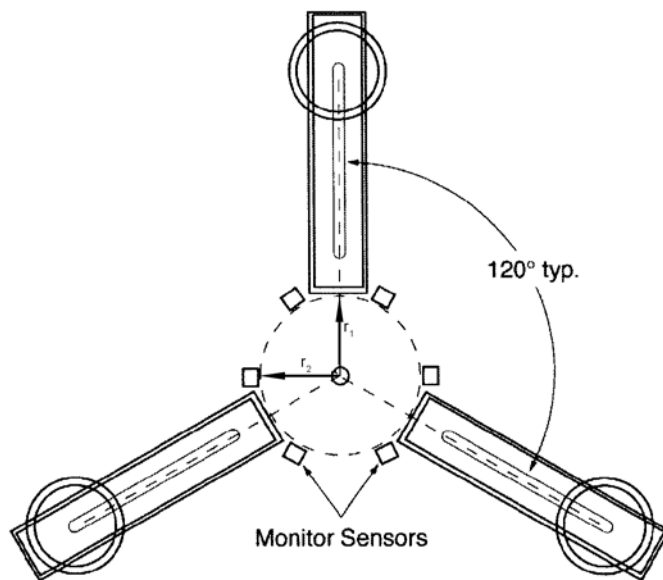
FIG. 1 Arrangement of Three Panel Sensors with Monitor Sen-
