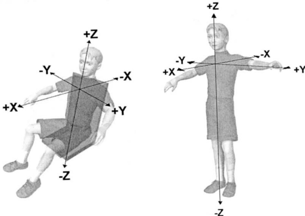
FIG. 2 Patron Coordinate System
