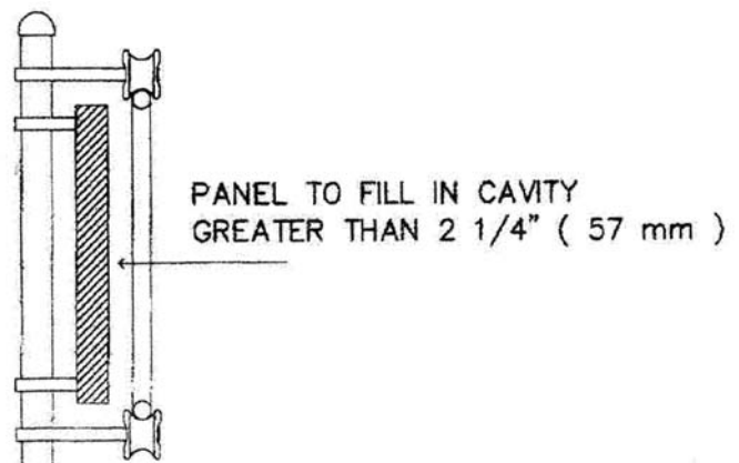
FIG. 1 Vehicular Horizontal Slide Gate Section
